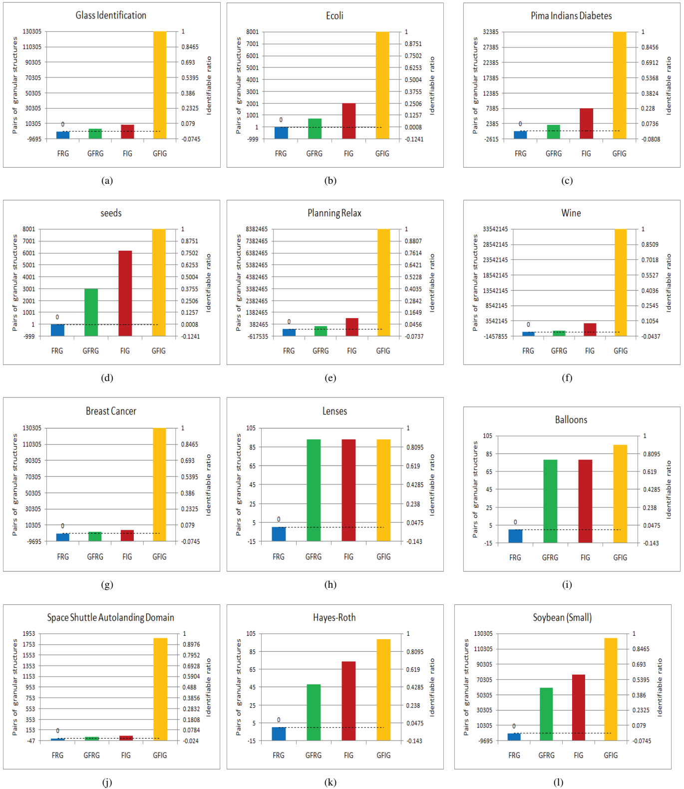
Fig. 3: Pairs of fuzzy granular structures distinguished by four different axiomatic approaches to fuzzy information granularity respectively and their Identifiable ratios on twelve data sets
