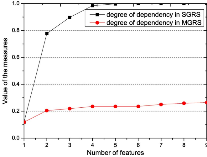
Fig. 4. Variation of the 2^\circ of dependence with the numbers of features (data set breast-cancer-wisconsin).
